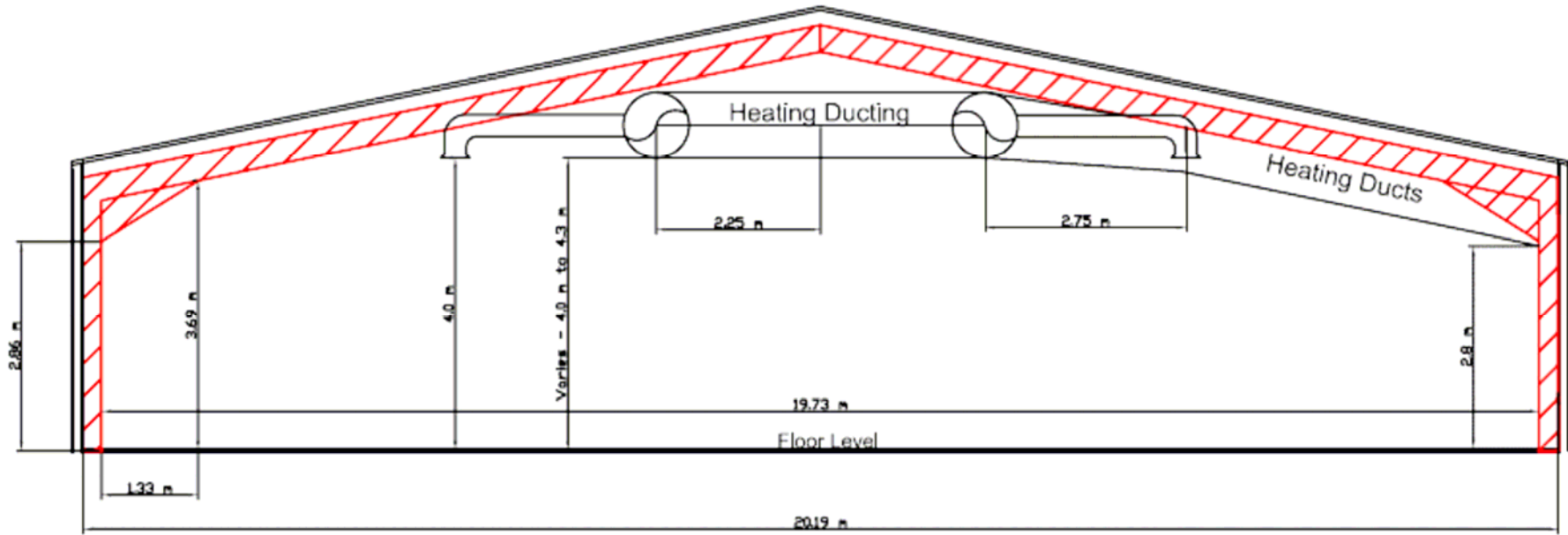
Hall B Steelwork and Heating Duct Dimensions (viewed from Ripon Road end)
